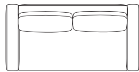
MD-805-2P W1800×D900×H750 (SH380) AH530
